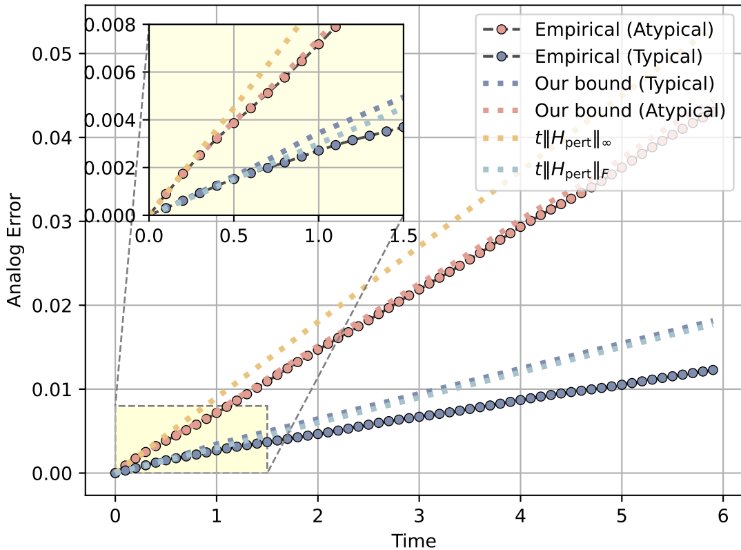
QIMF, long-time evolution with imperfections
